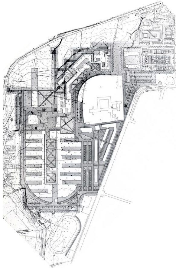
PLAN OF STREETS AND EXTERIOR ARRANGEMENTS ALCINO SOUTINHO - 1989
